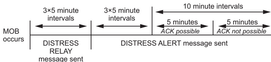
Example of OPEN mode transmission intervals
